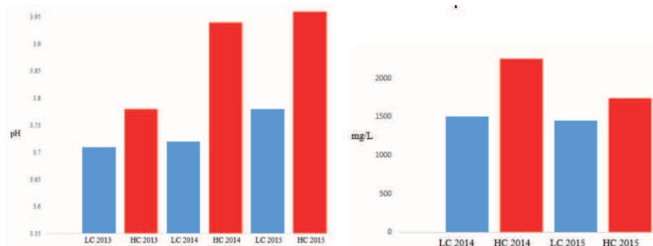
Figure 3: Bar graphs showing the pH and potassium concentrations of the final experimental wines. The LC wine consistently shows lower K concentration and lower pH than the HC wine. Note that only pH values for the 2013 wines are provided as K ++ analysis was not initiated for this study until the 2014 vintage.
